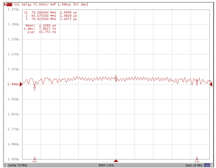
Group Delay Variation F_o \pm 6.925\text{MHz}
