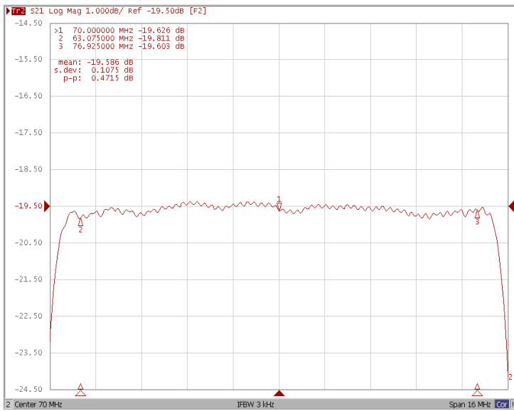
Ripple Variation F_o \pm 6.925\text{MHz}
